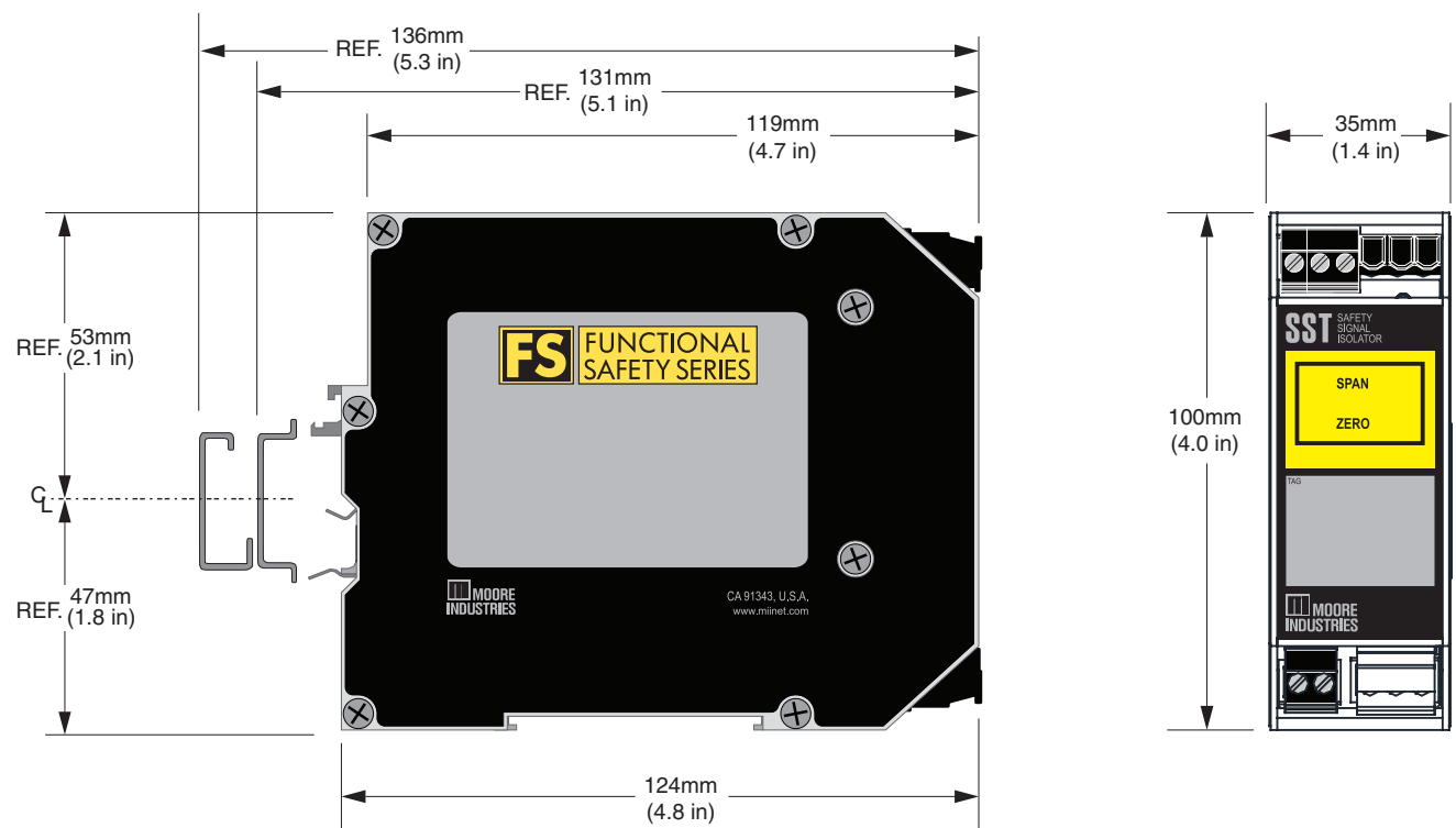
Figure 10. Dimensions of the SST Isolator in its aluminum DIN-style housing
