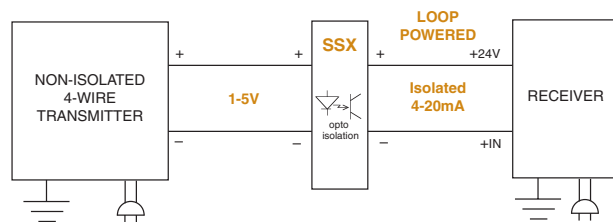
Figure 5. The SSX solves bucking power supplies. Also, when used with the -0HART option, the SSX acts as a current isolator that stops a HART signal from reaching a PLC, DCS or other receiving device.
