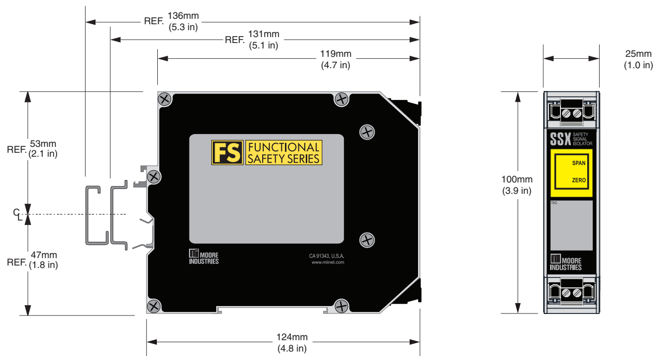
Figure 9. Dimensions of the SSX Isolator in its aluminum DIN-style housing
