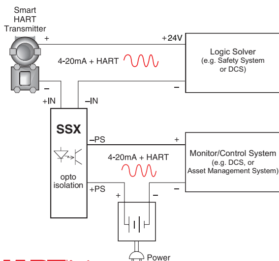
Figure 1. The 2-wire SSX provides safety system isolation while still allowing valuable HART data to pass.
