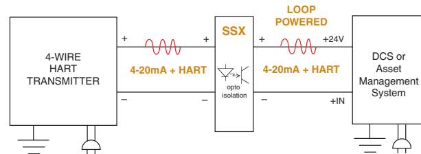
Figure 4. The SSX can also serve as a signal converter.
